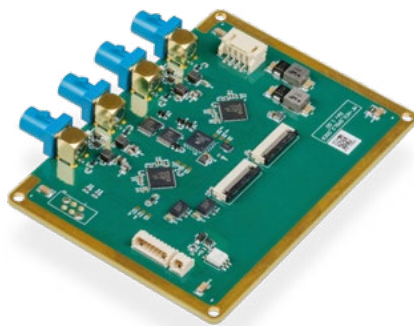
4-Channel GMSL2 (coming soon)
